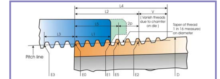
Fig. 5 (Taper)
